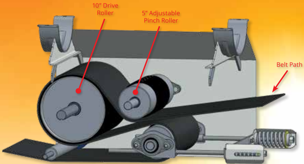
Spring Tension Pinch Drive Box, used on conveyors 52.5' and shorter
