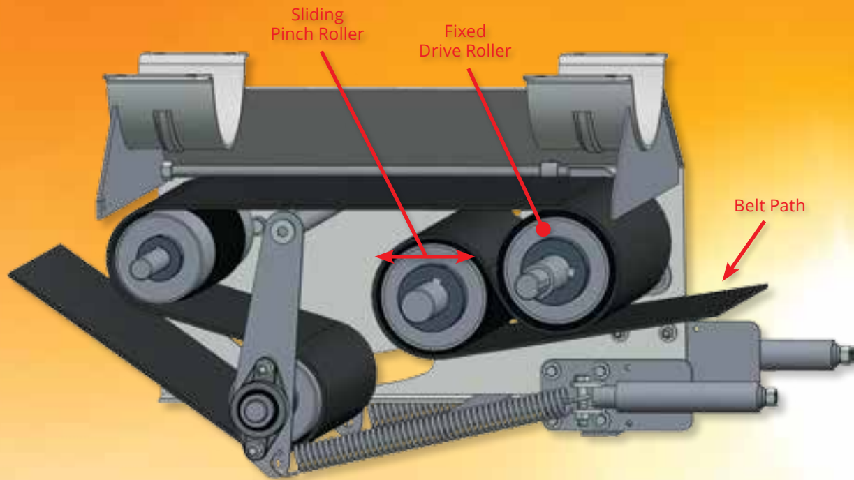
Positive Pinch Drive Box, used on conveyors 55' and longer
